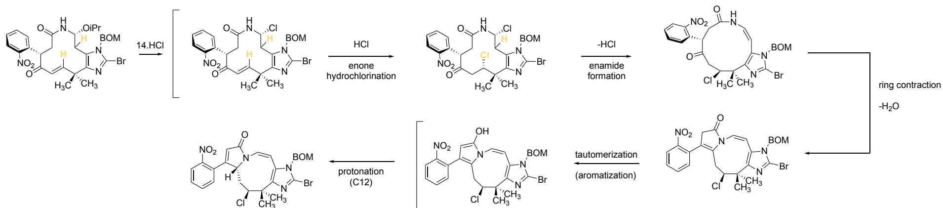
Step 14 mechanism step by step
