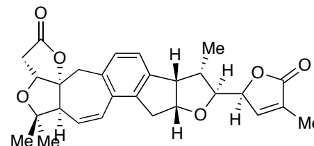
Rubriflordilactone B
