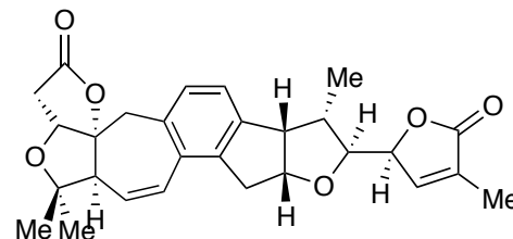
Rubriflordilactone B
