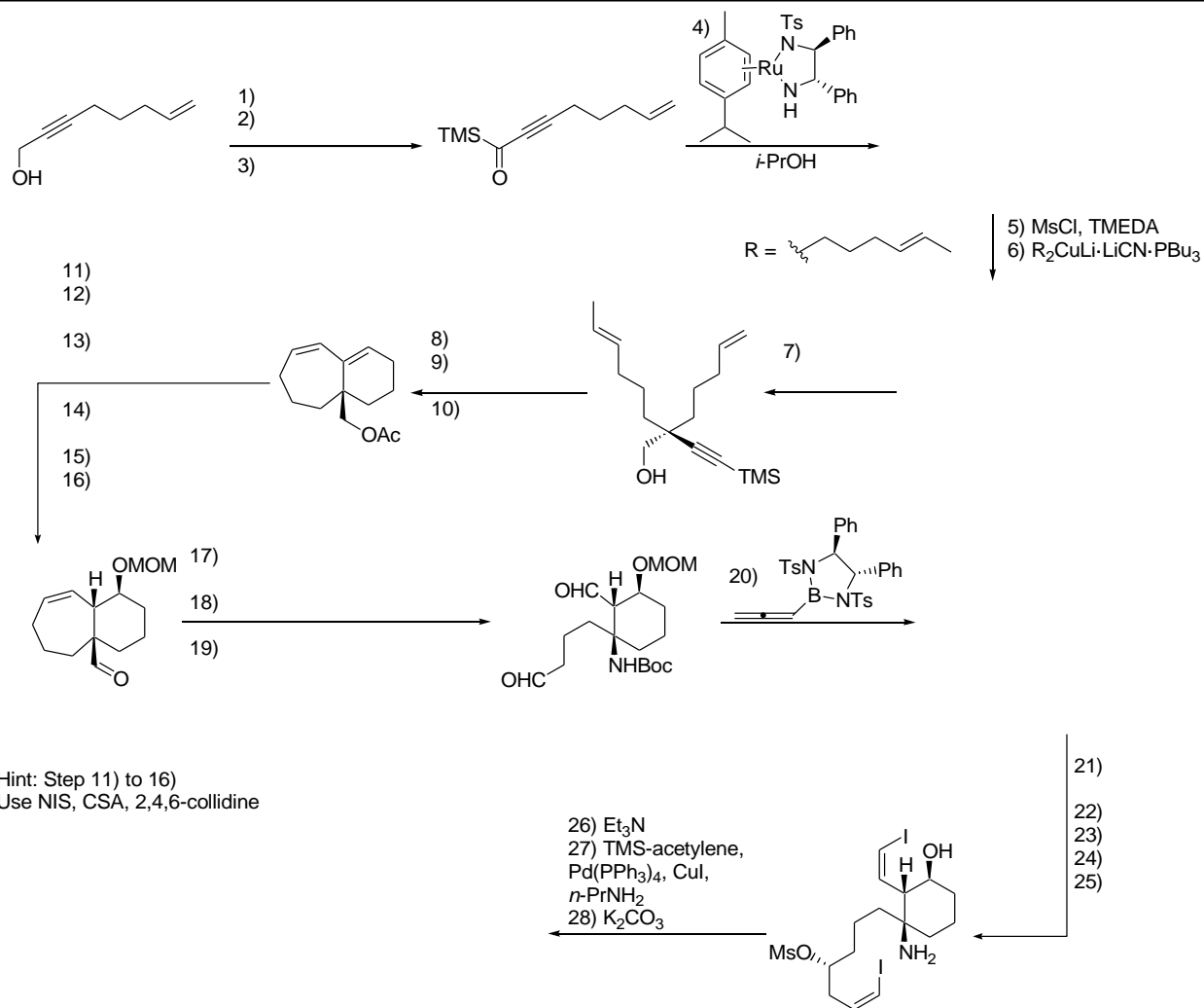
(-)-histrionicotoxin
