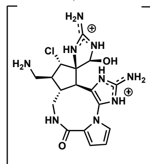
"macro-palau'amine"
