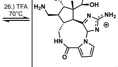
amidine tautomer
