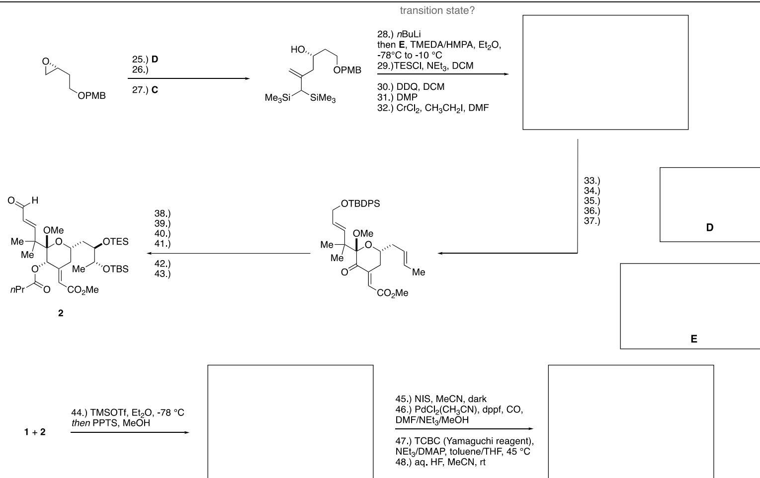
Bryostatin 8
